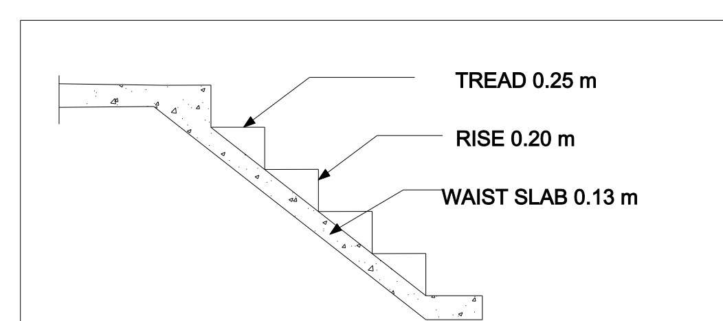
STAIR DETAILS
