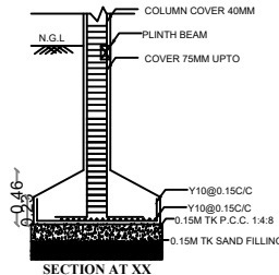
SECTION AT XX
