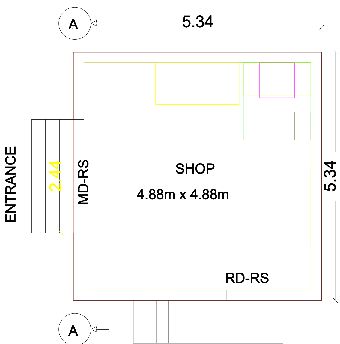
FLOOR PLAN
