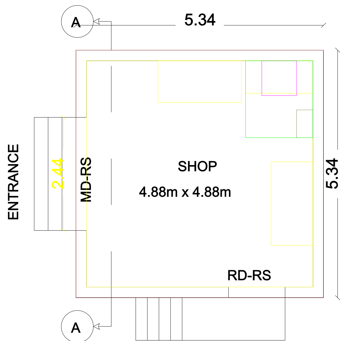
FLOOR PLAN
