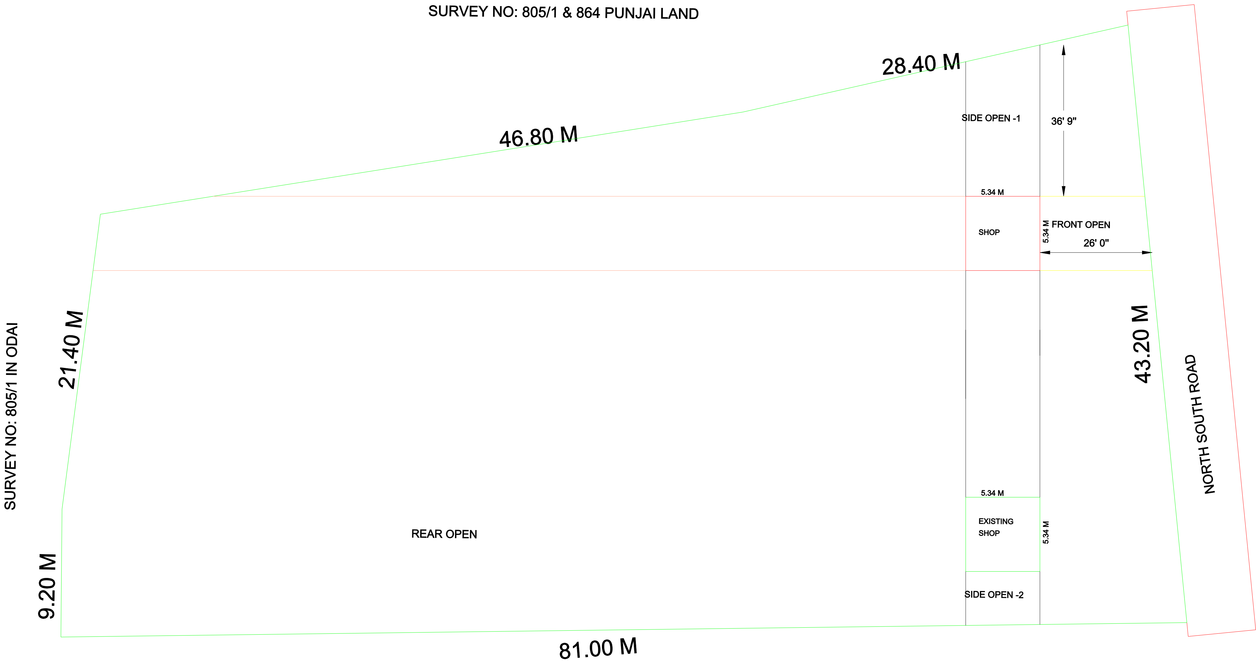
SITE PLAN
