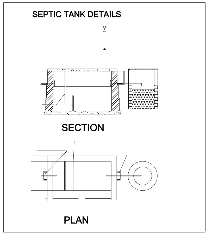
PLAN
