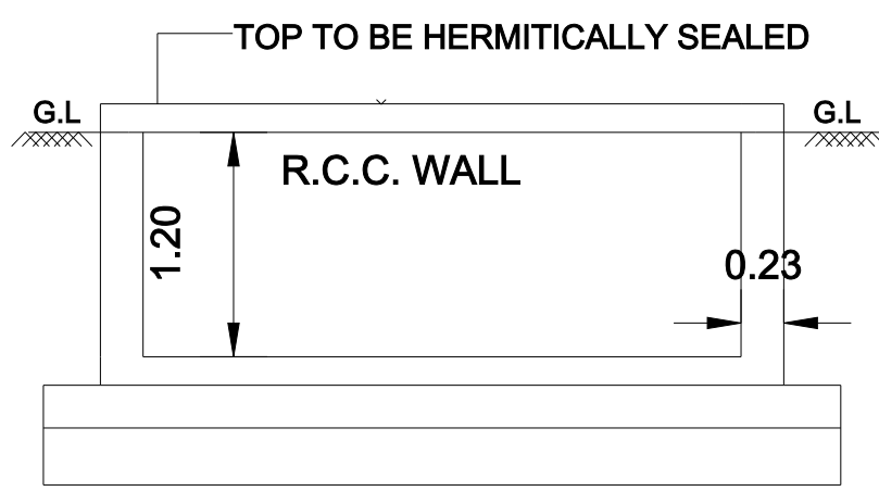
RWI SECTION ( SAMPLE)
