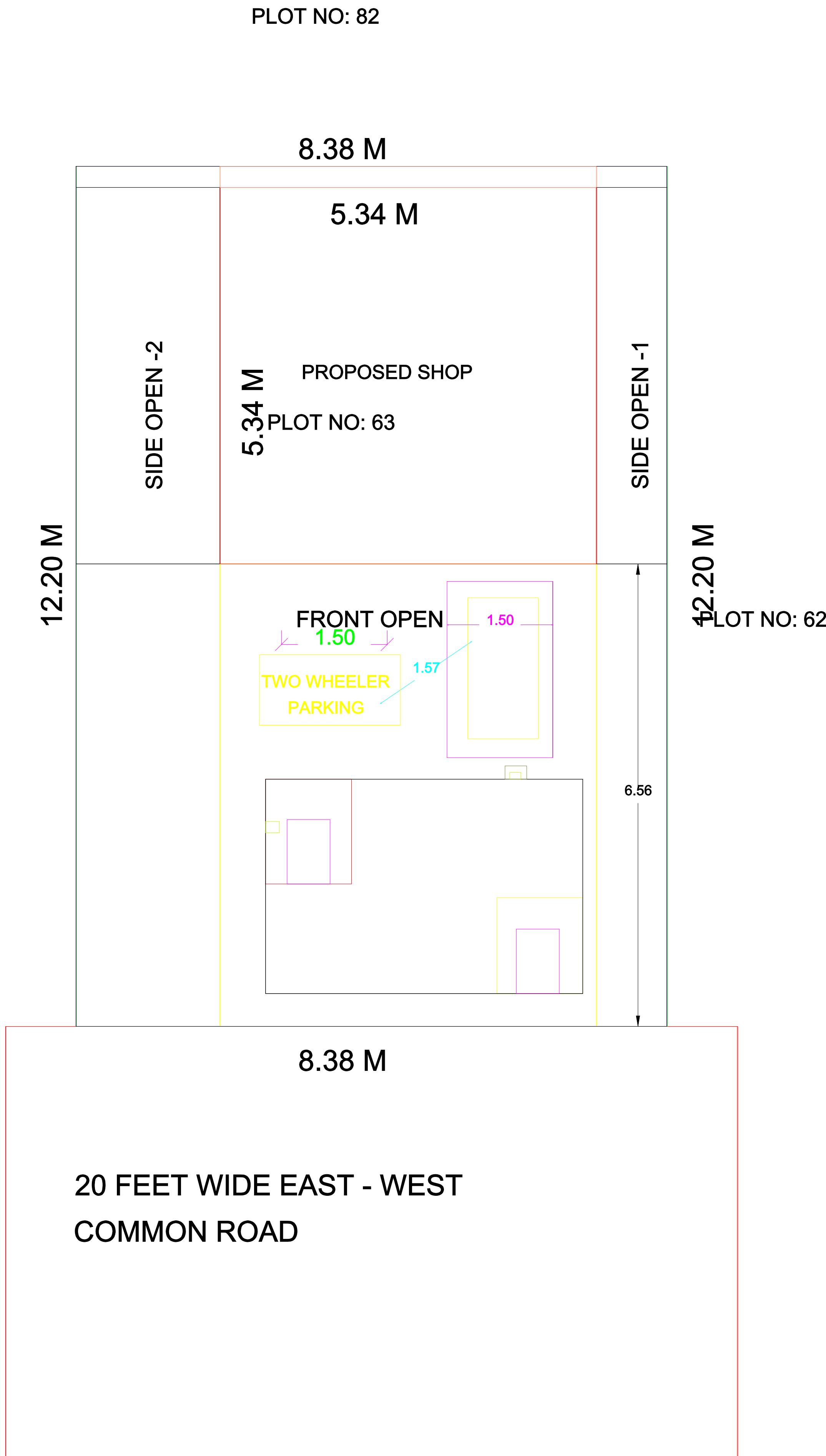
SITE PLAN
