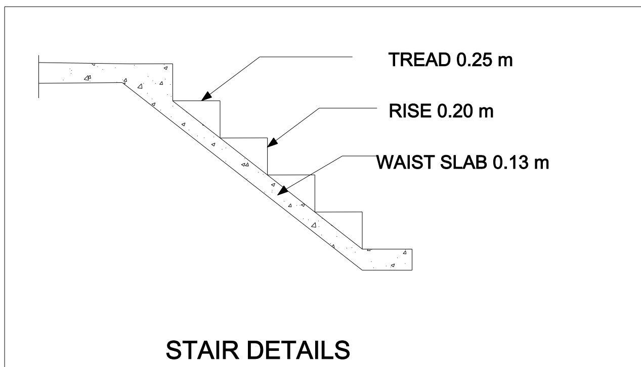
STAIR DETAILS
