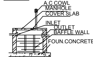
DETAILS OF SEPTIC TANK
