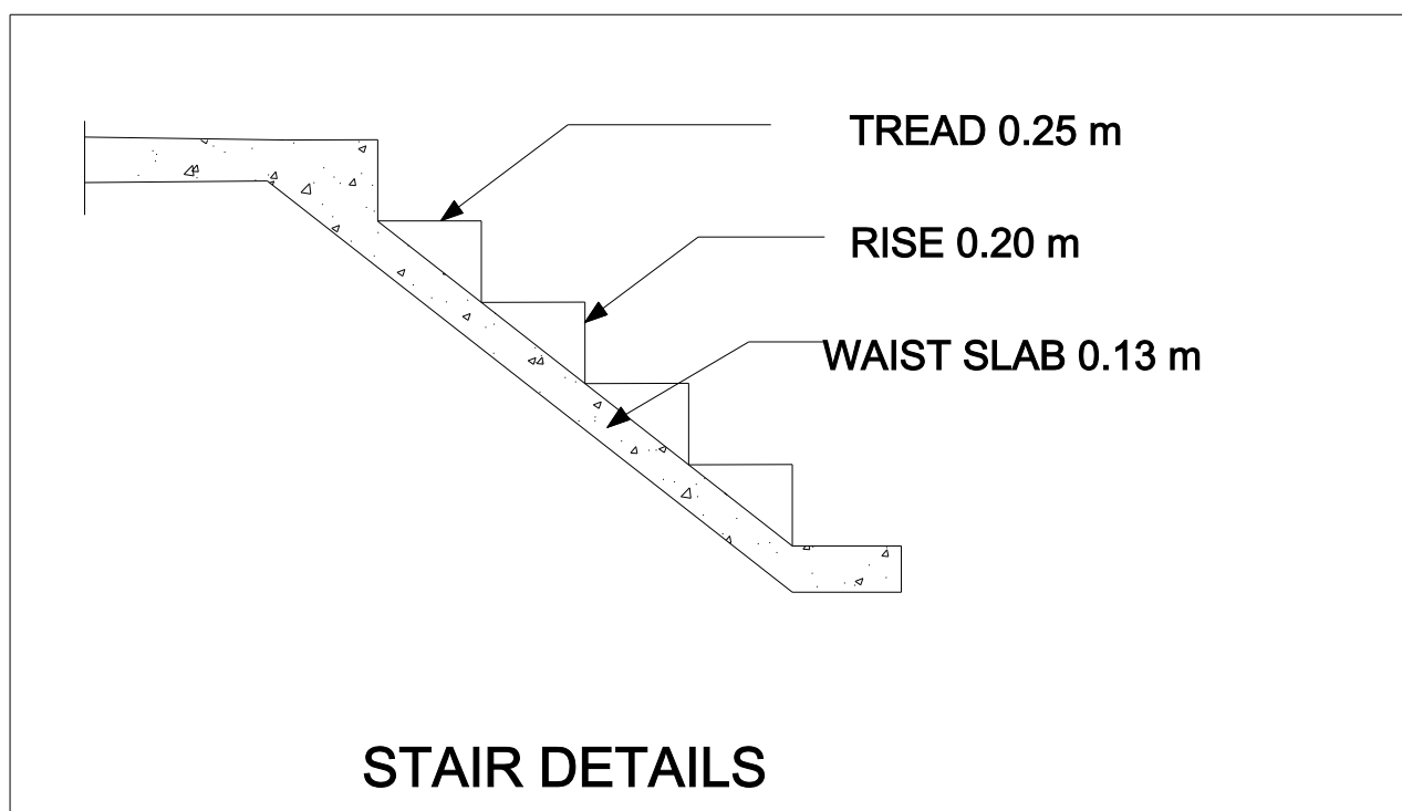
STAIR DETAILS
