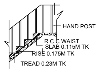
DETAILS OF STAIRCASE
