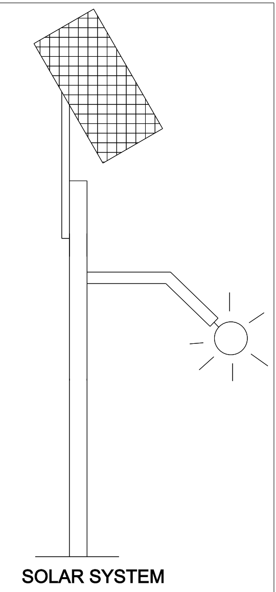
SOLAR SYSTEM
