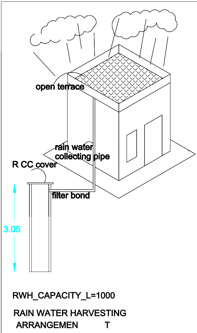
RAIN WATER HARVESTING ARRANGEMENT
