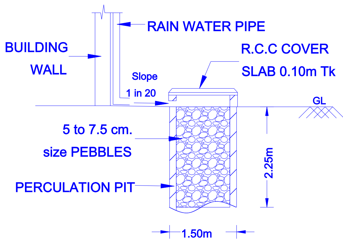
RAIN WATER HARVESTING TRENCH PIT DETAILS
