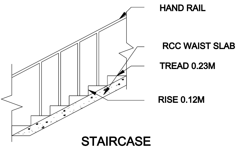
STAIRCASE
