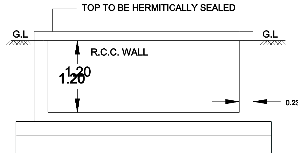
RWH SECTION
