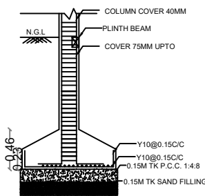
SECTION AT XX
