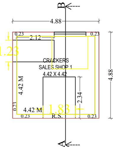
GROUND FLOOR PLAN-1
