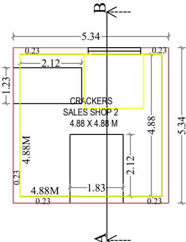
GROUND FLOOR PLAN-2
