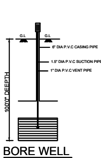
BORE WELL
