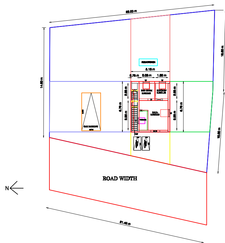
1D FLOOR PLAN
