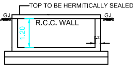
RWH SECTION ( SAMPLE) RWH_CAPACITY_L=2000
