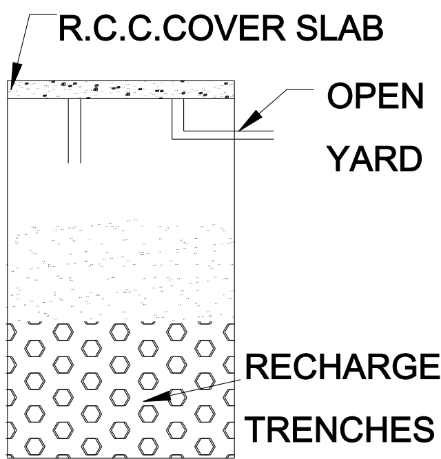
SECTION
