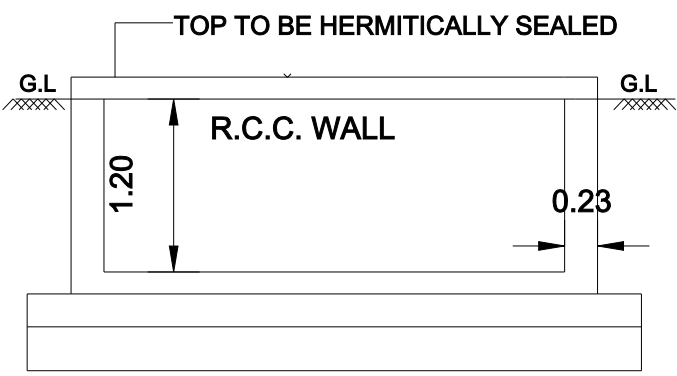
RWH SECTION ( SAMPLE)
