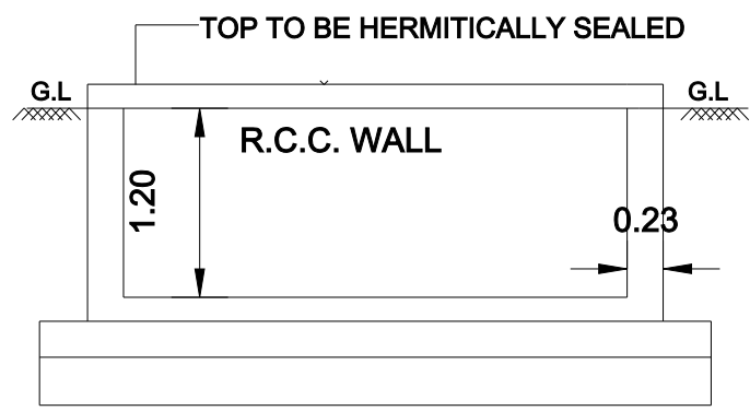
RWH SECTION ( SAMPLE)
