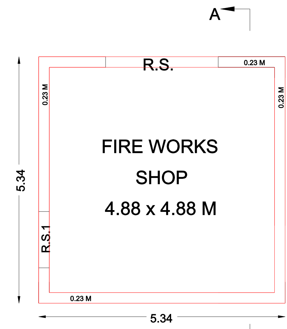
PROPOSED FIRE WORKS SHOP
