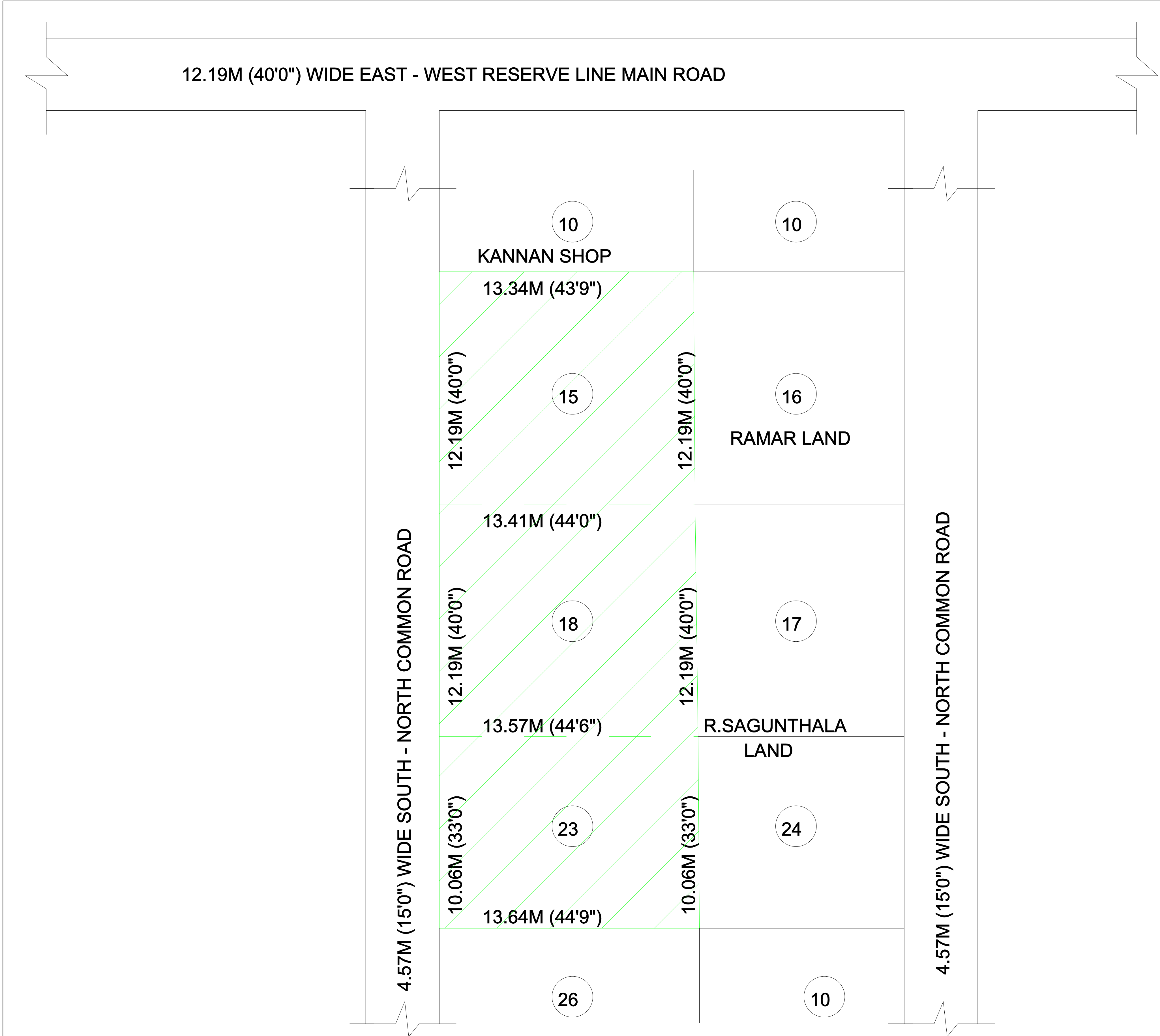
LOCATION PLAN
