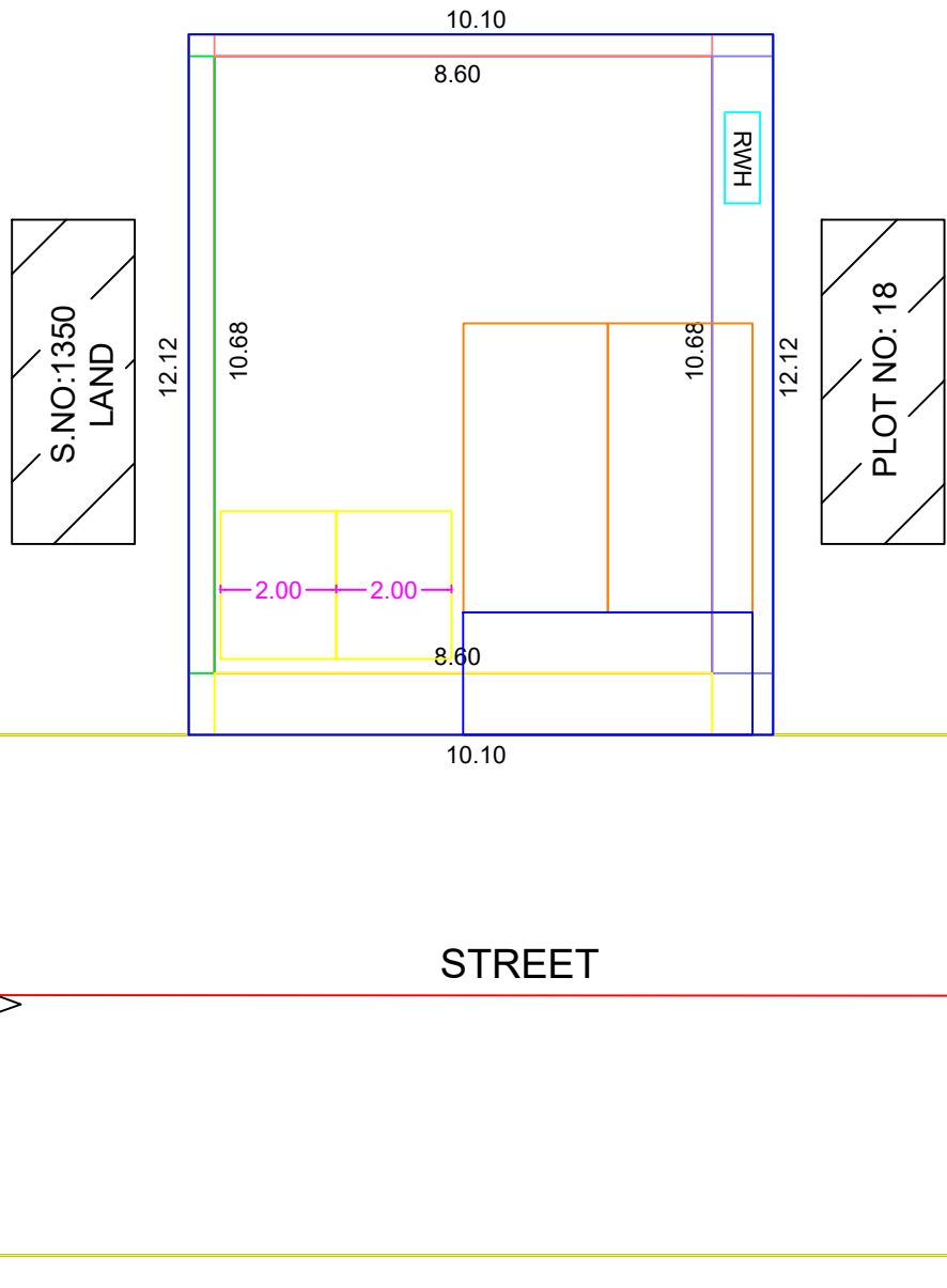
TOPO PLAN Scale 1:100
