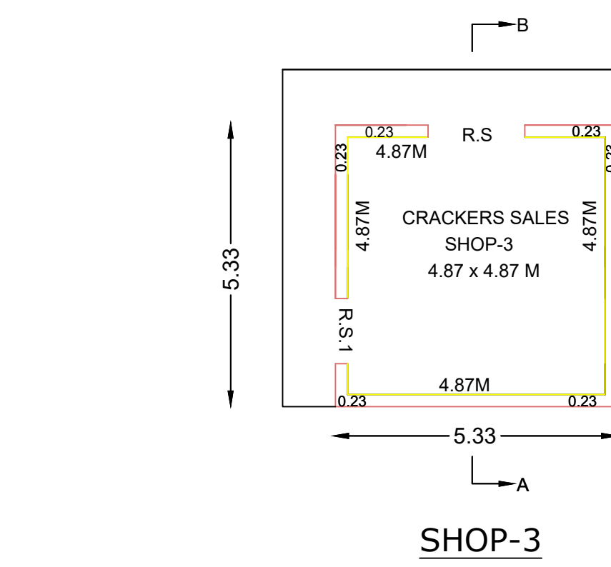
SHOP-3
