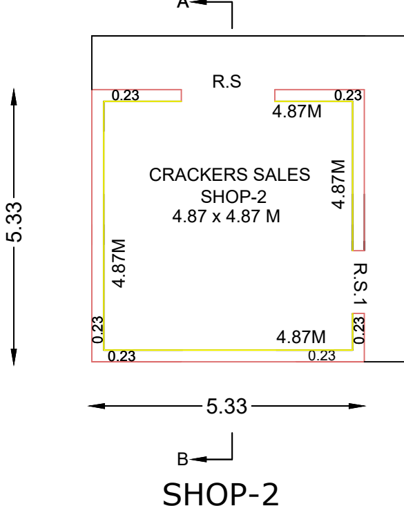
SHOP-2
