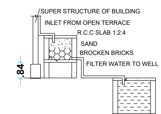
RAINWATER HARVESTING
