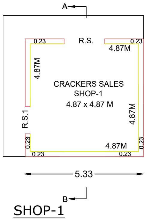
SHOP-1
