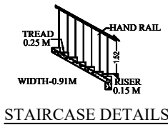
STAIRCASE DETAILS
