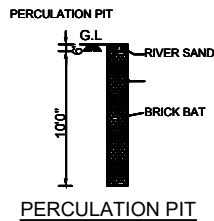
PERCOLATION PIT
