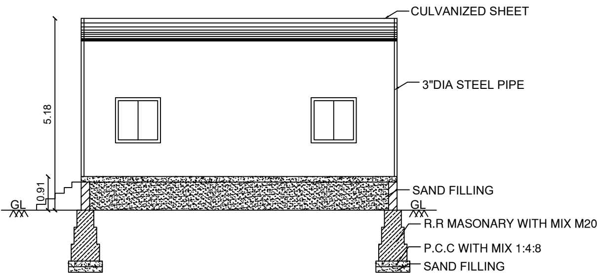
SECTION ON "BB"
