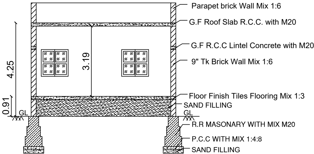
SECTION ON "CC"
