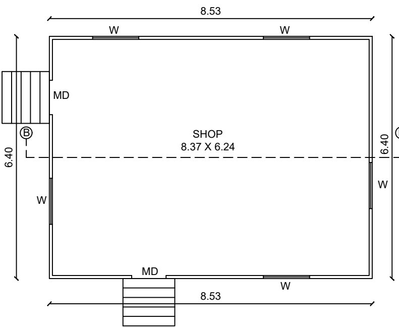
BLOCK-2 GROUND FLOOR PLAN
