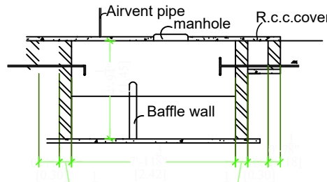
SEPTIC TANK DETAILS (NTS)
