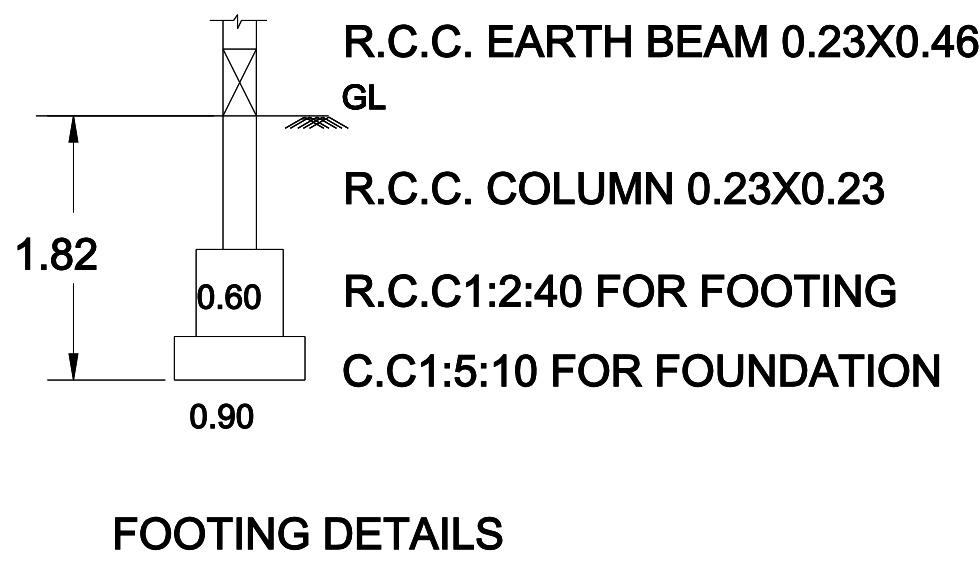
FOOTING DETAILS
