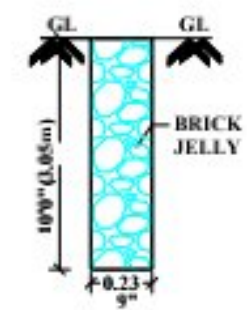
PERCOLATION PIT
