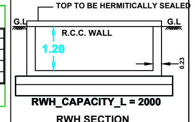
RWH SECTION
