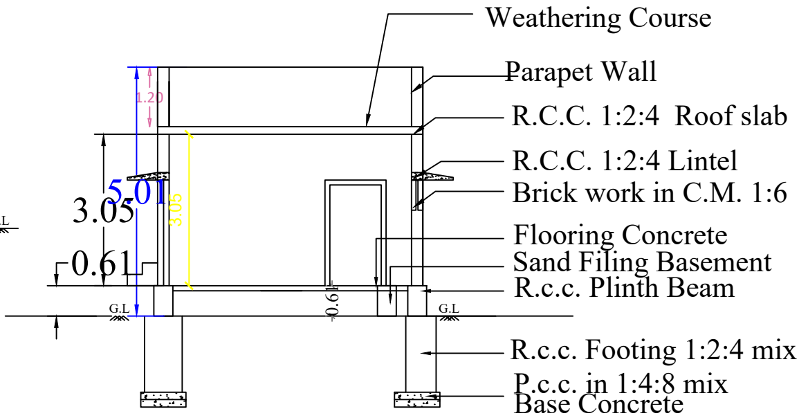
SECTION -"AB"
