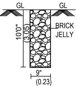
PERCOLATION PIT:-
