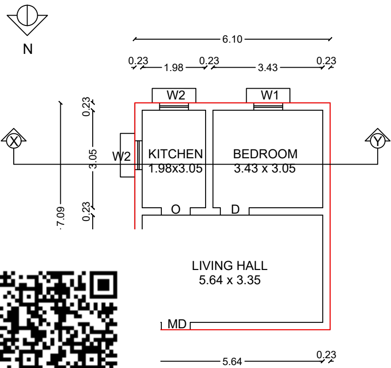
D GROUND FLOOR PLAN
