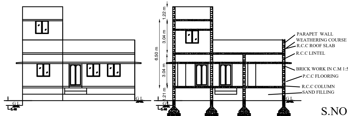
FRONT ELEVATION
