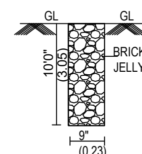
PERCULATION PIT:-
