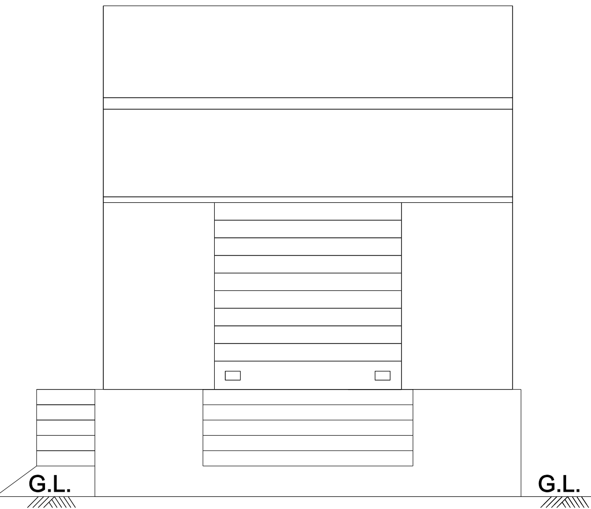
FRONT ELEVATION
