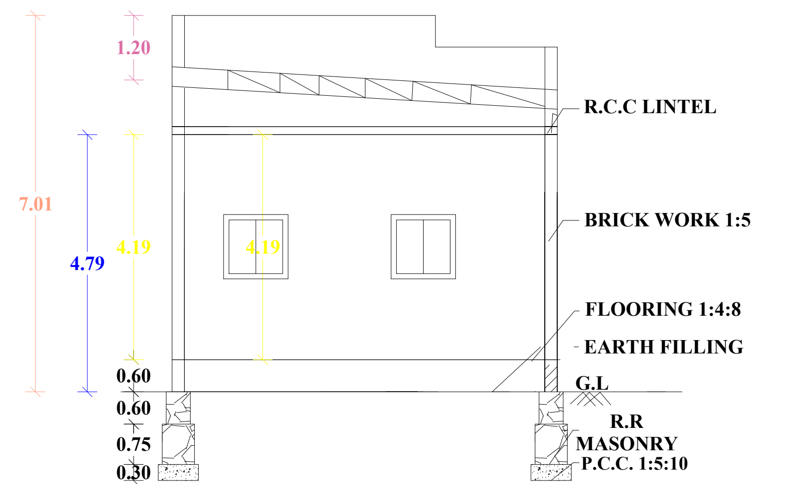
"SECTION "AB"
