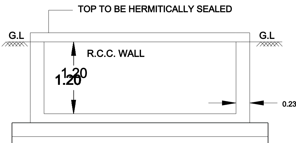
RWH SECTION RW_H_CAPACITY_L = 2000
