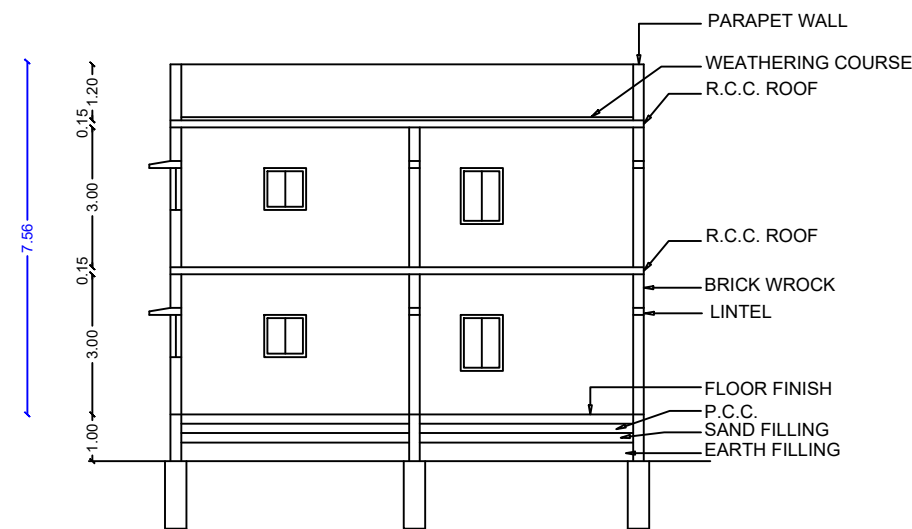
SECTION ON "XY"
