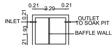
PLAN SEPTIC TANK
