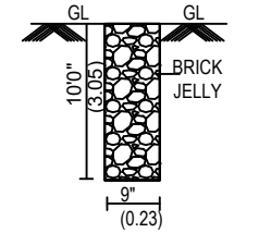
PERCOLATION PIT:-
