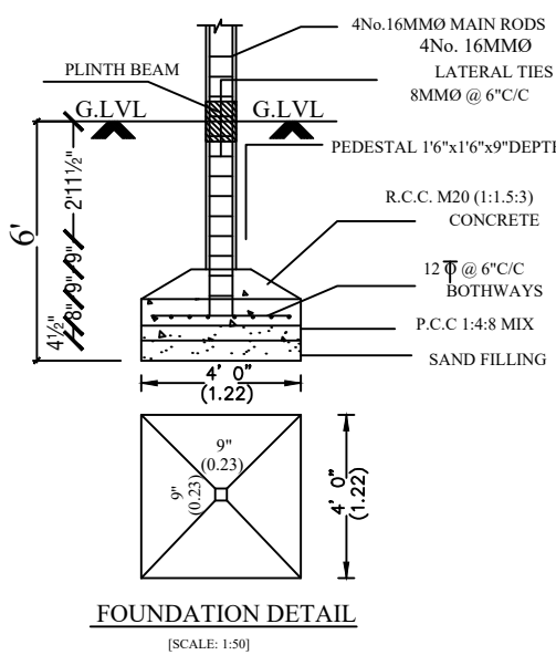
FOUNDATION DETAIL
