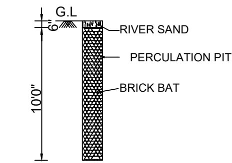
PERCOLATION PIT
