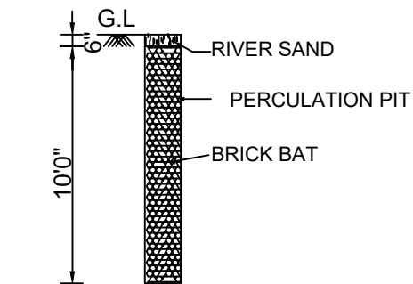
PERCULATION PIT
