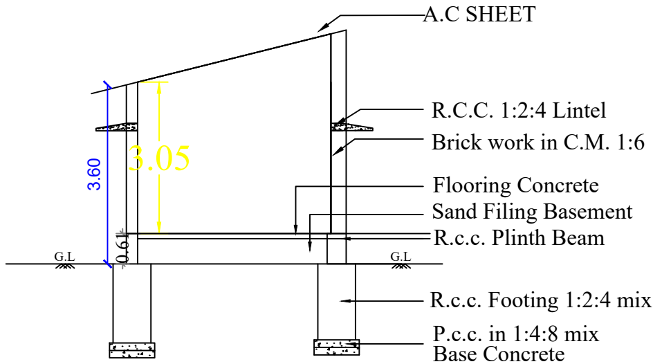
SECTION -"AB"
