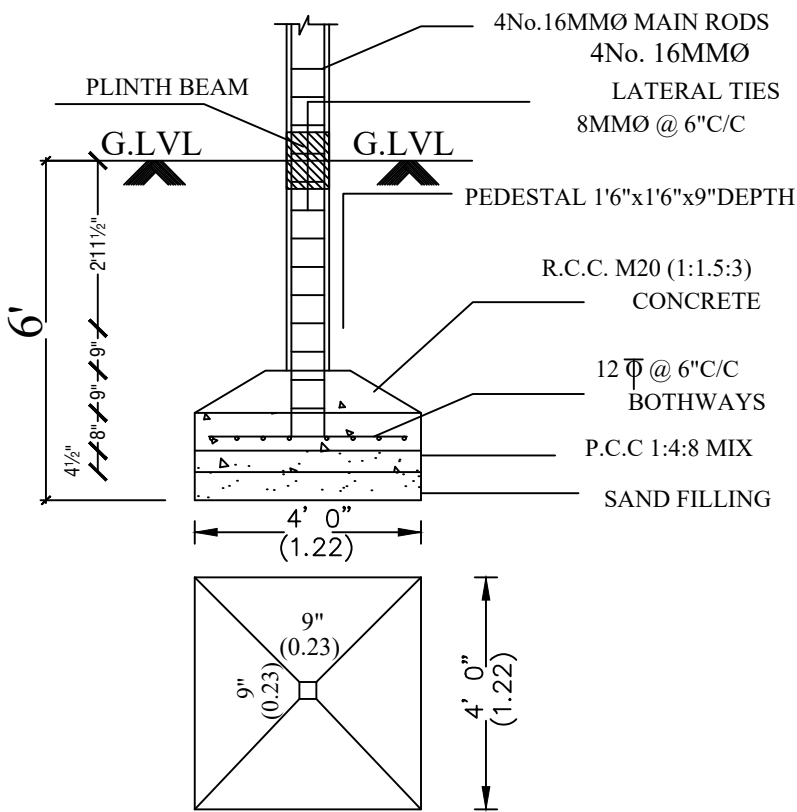
FOUNDATION DETAIL
