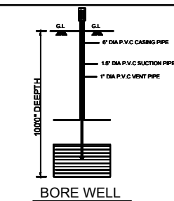
BORE WELL
