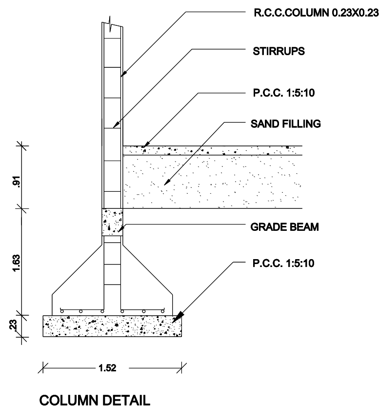
COLUMN DETAIL
