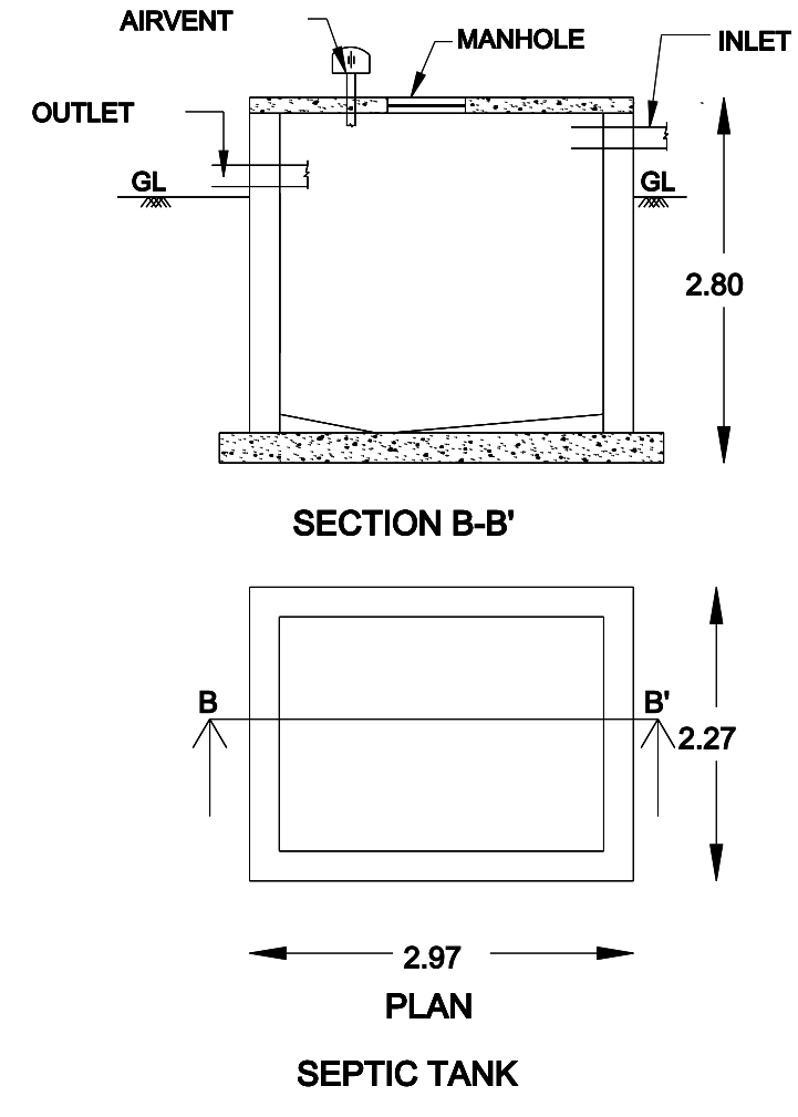
SEPTIC TANK
