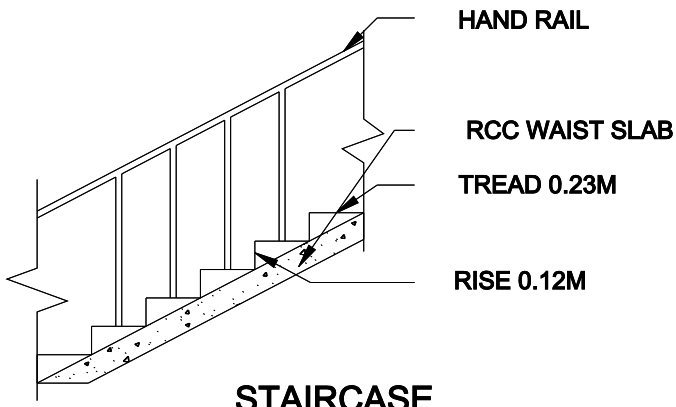
STAIRCASE
