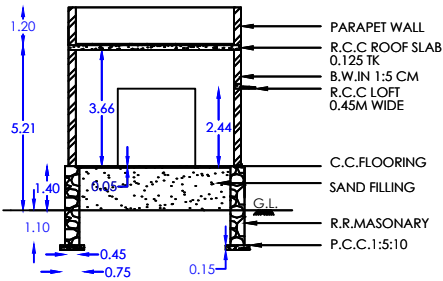
SECTION ON-AB
