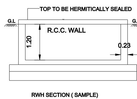
RWH SECTION ( SAMPLE)
