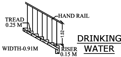
STAIRCASE DETAILS
