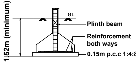
TYP.DET.COLUMN FOOTING
