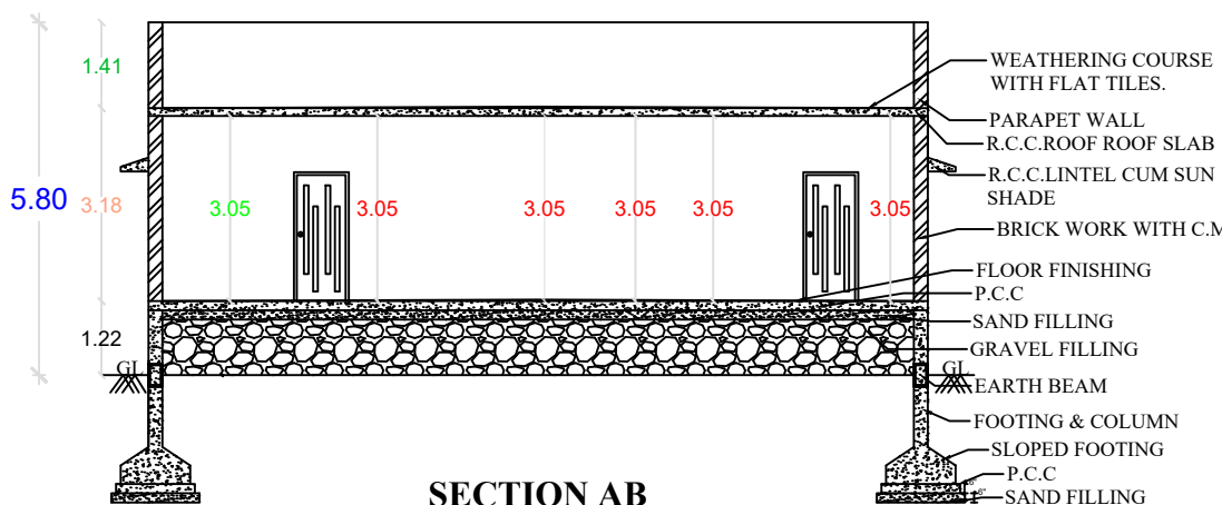
SECTION AB
