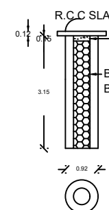
PERCOLATION PIT
