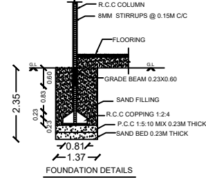
FOUNDATION DETAILS
