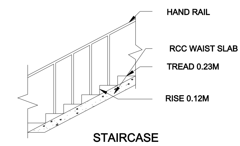
STAIRCASE
