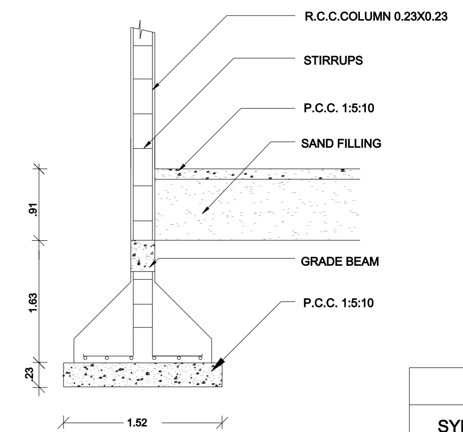
COLUMN DETAIL
