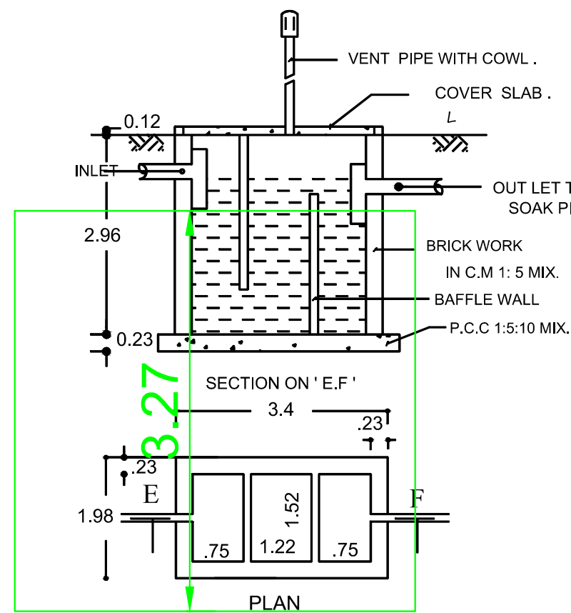
SEPTIC TANK DETAILS ( NOT TO SCALE )
