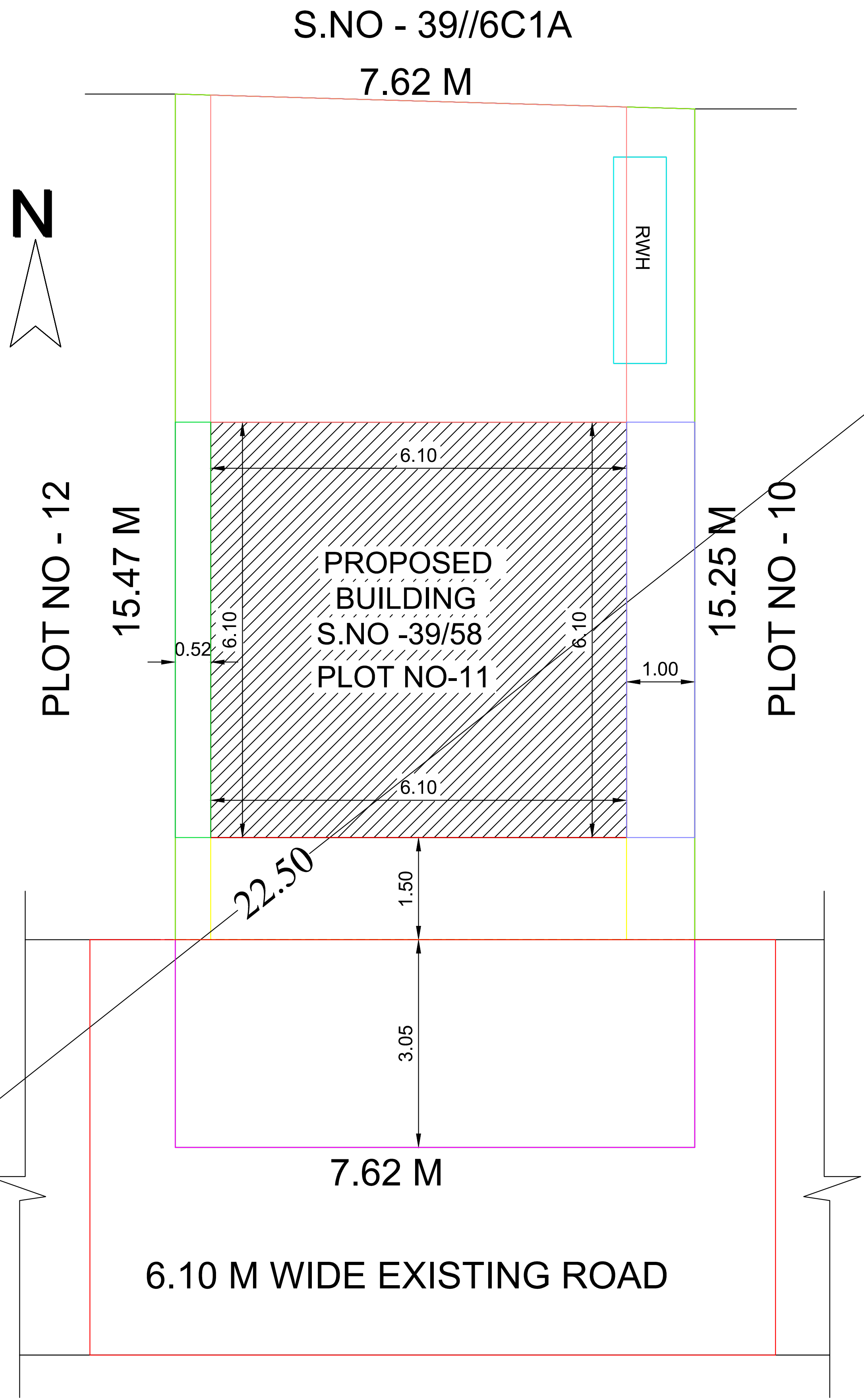
SITE PLAN
